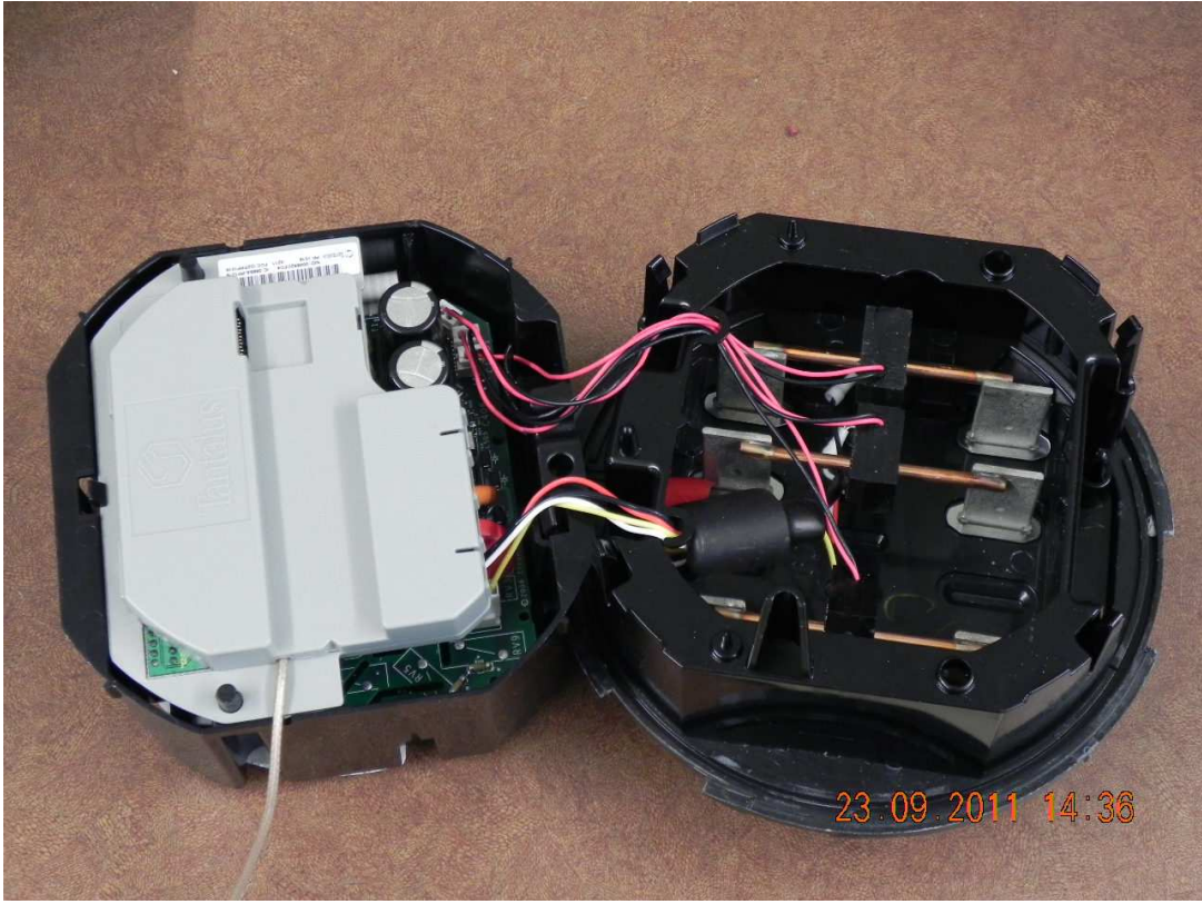
Assembled PP1316 – Internal View
