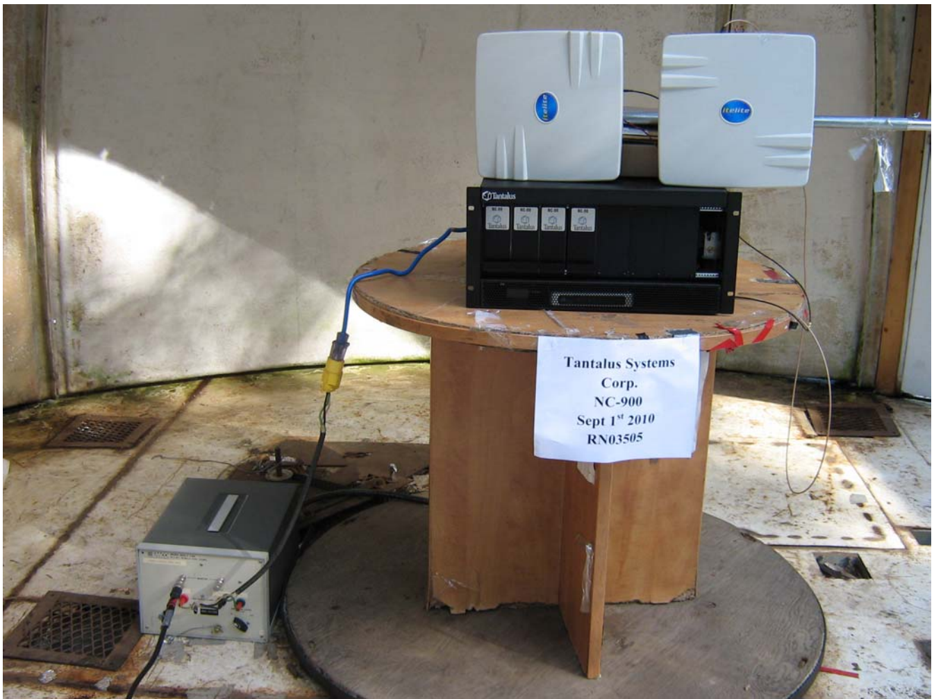
AC Conducted Test Setup – Front View
