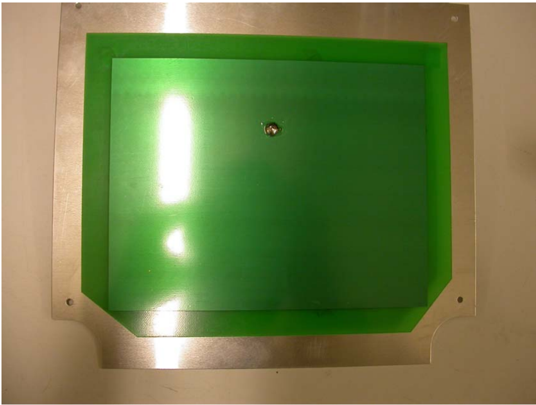
RX Patch Antenna View (Front)
