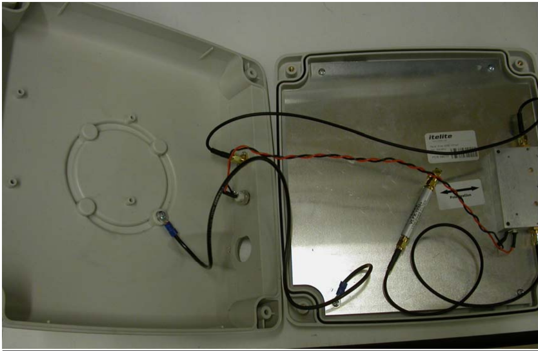
TX Antenna Internal View
