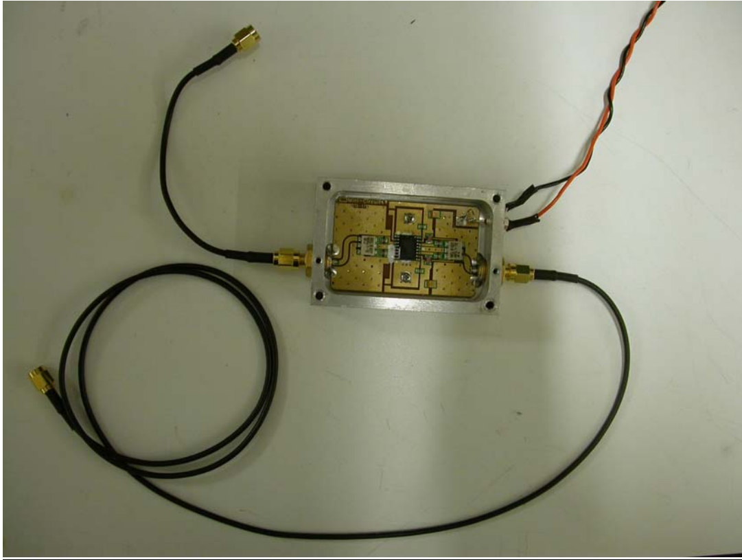
TX Power Amplifier (Front)
