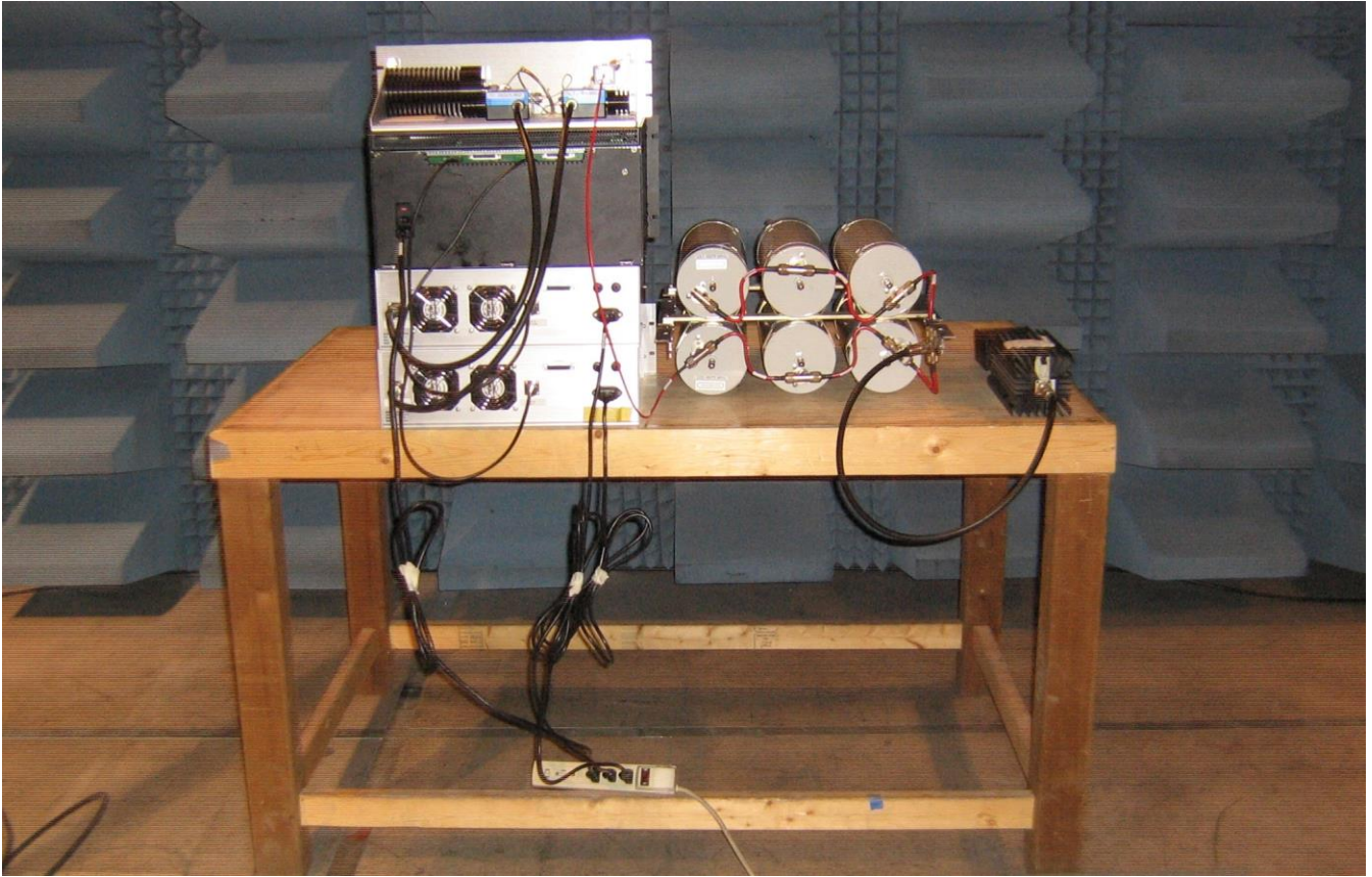
RF Conducted Test Setup
