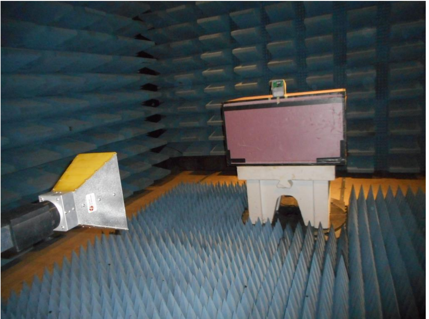
Emissions Test Setup – Intentional Radiated Emissions 1000 - 10000 MHz
