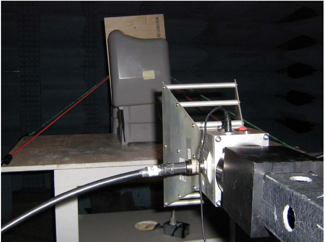
Intentional Radiated Emmissions 1000 – 10000 MHz setup.
