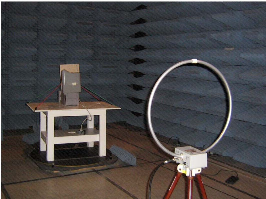
Intentional / Unintentional Radiated Emission 0.009 – 30 MHz setup. Emissions Test Setup – Intentional / Unintentional Radiated Emissions
