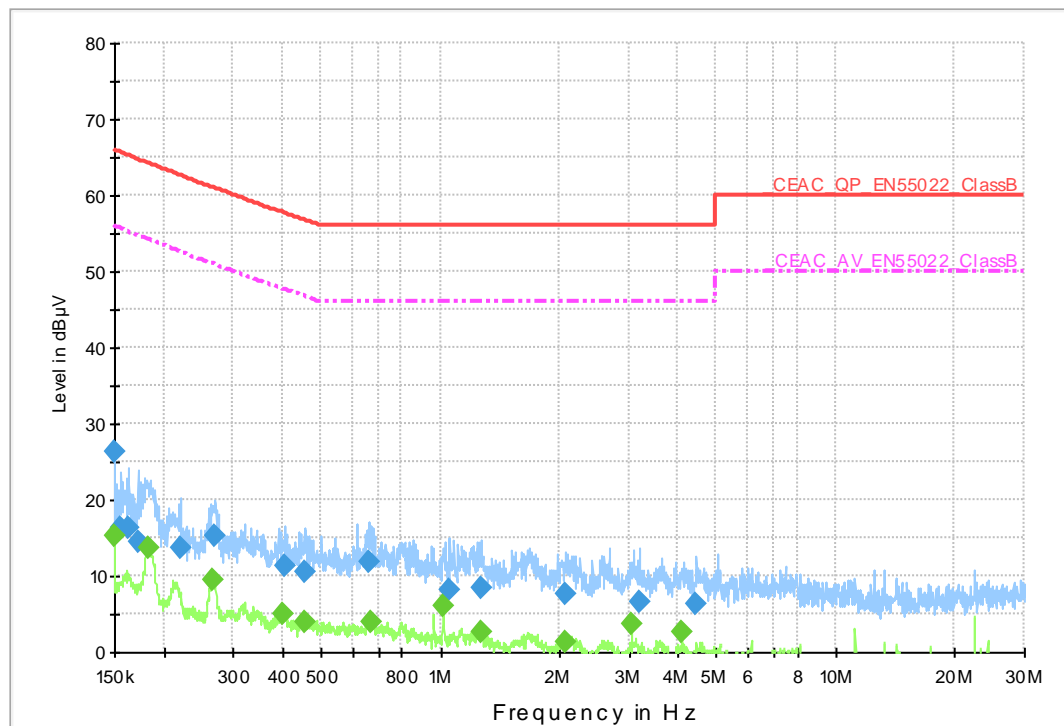
Figure 1: 120V AC Conducted Emissions - Line 1 and Line 2
