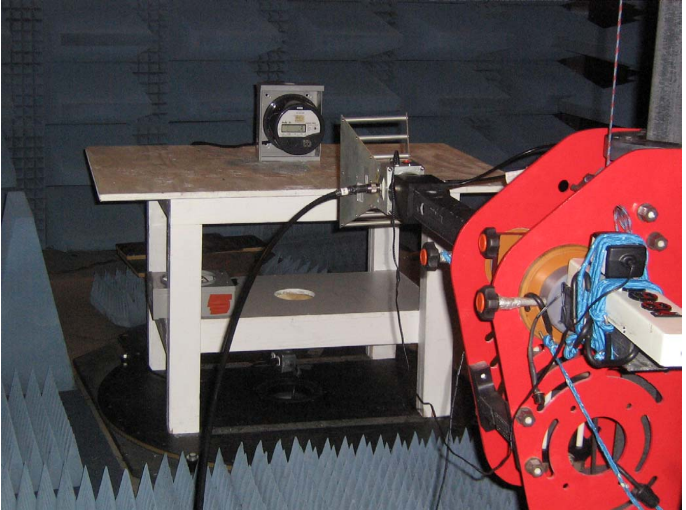
Emissions Test Setup – Intentional/Unintentional Radiated Emissions 1000 - 10000 MHz
