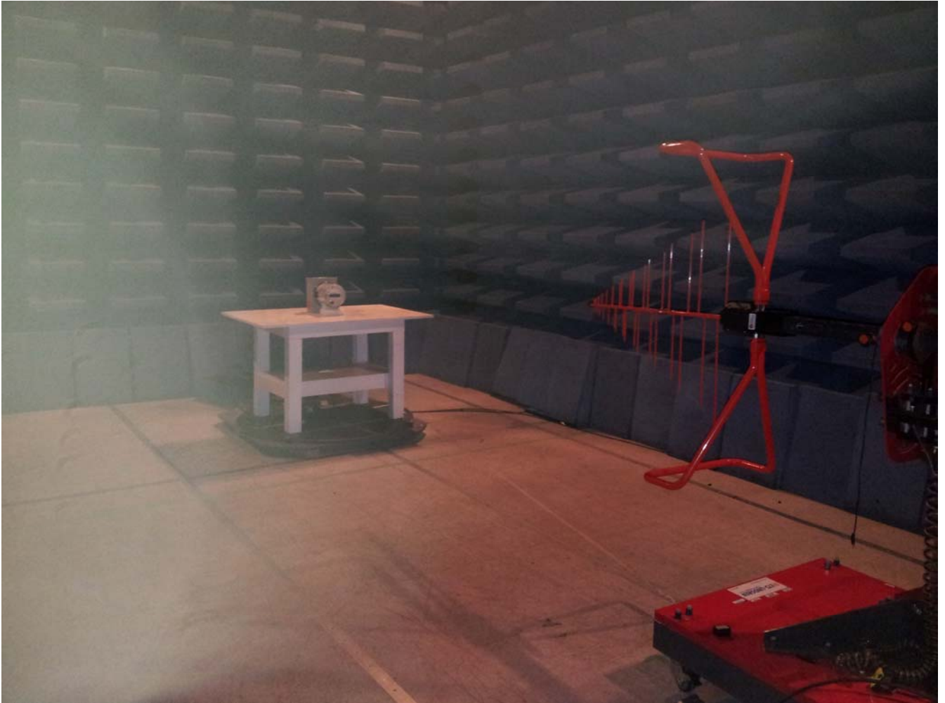
Emissions Test Setup – Intentional/Unintentional Radiated Emissions 30 – 1000 MHz
