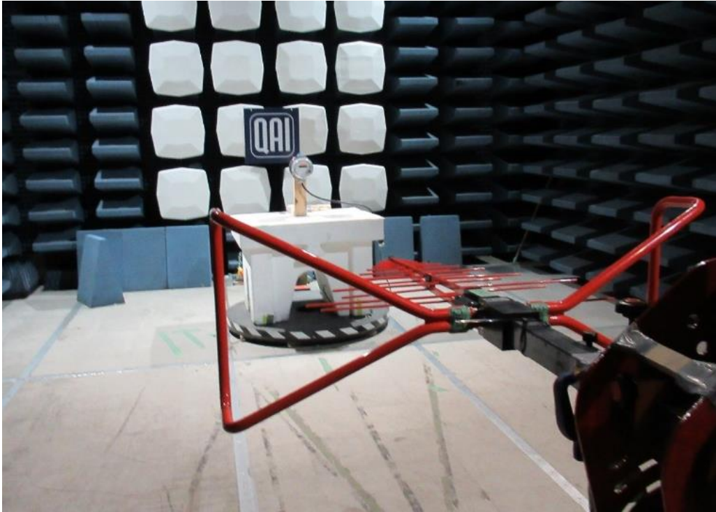
Emissions Test Setup – Unintentional Radiated Emissions 30 – 1000MHz
