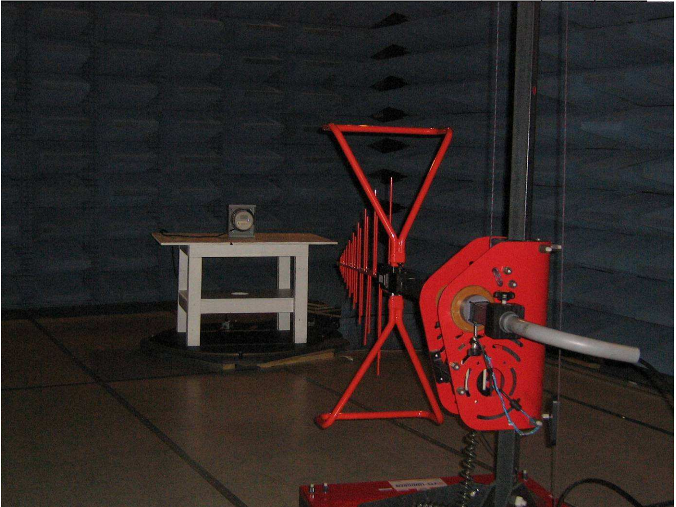
Figure 20 – Emissions Test Setup – Unintentional Radiated Emissions, 240V Figure 3: Emissions Test Setup – Radiated Emissions – I-210 240V
