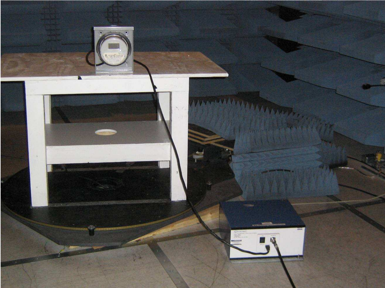
Figure 19 — OATS AC Conducted Test Setup Figure 1: OATS AC Conducted Test Setup – I-210
