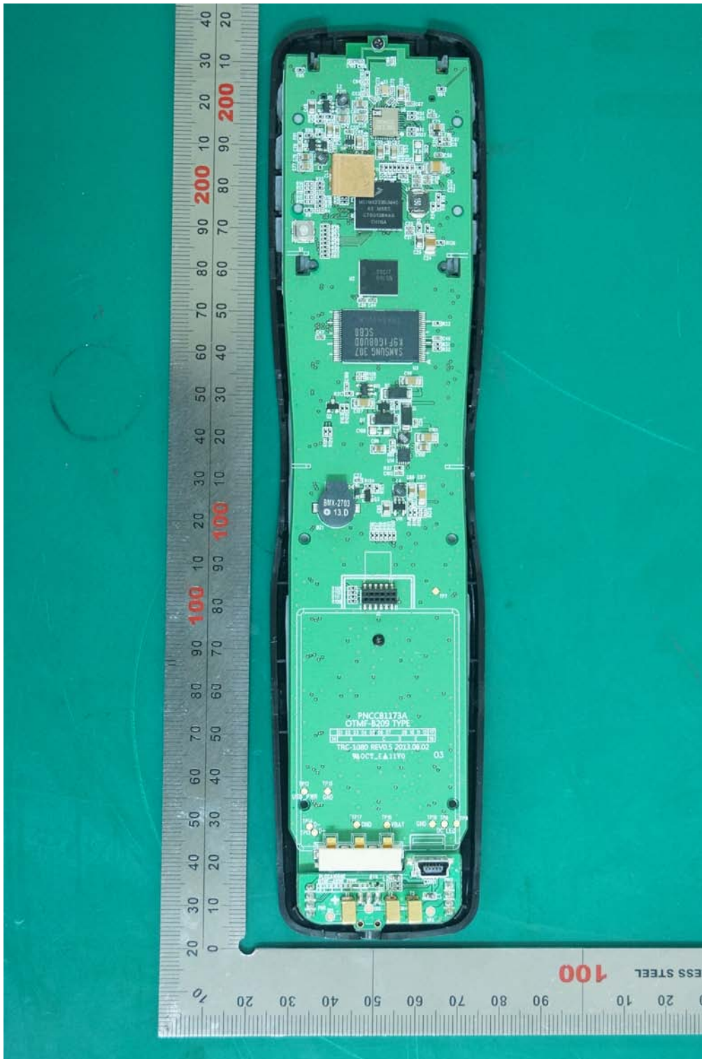
< Inside >
