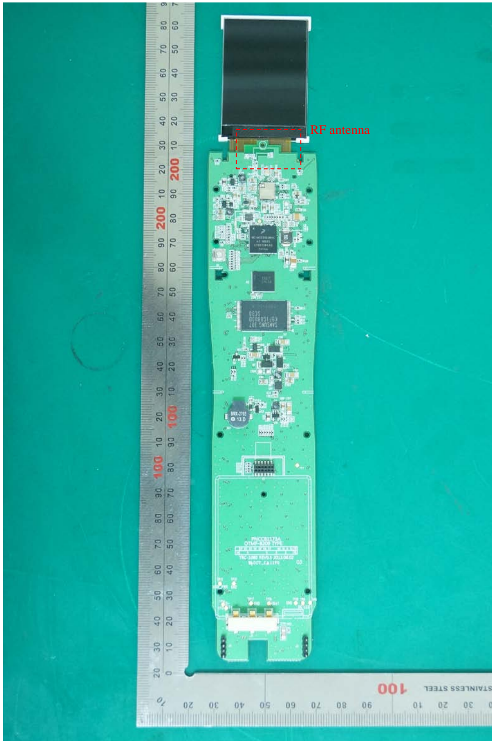
< Main board & LCD panel front >
