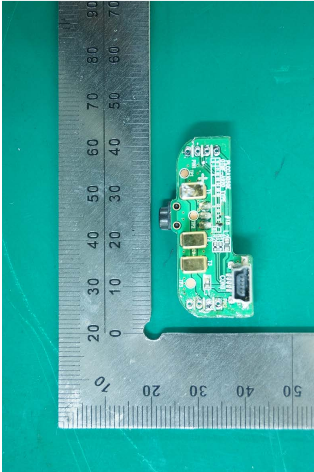
< SMPS Front >
