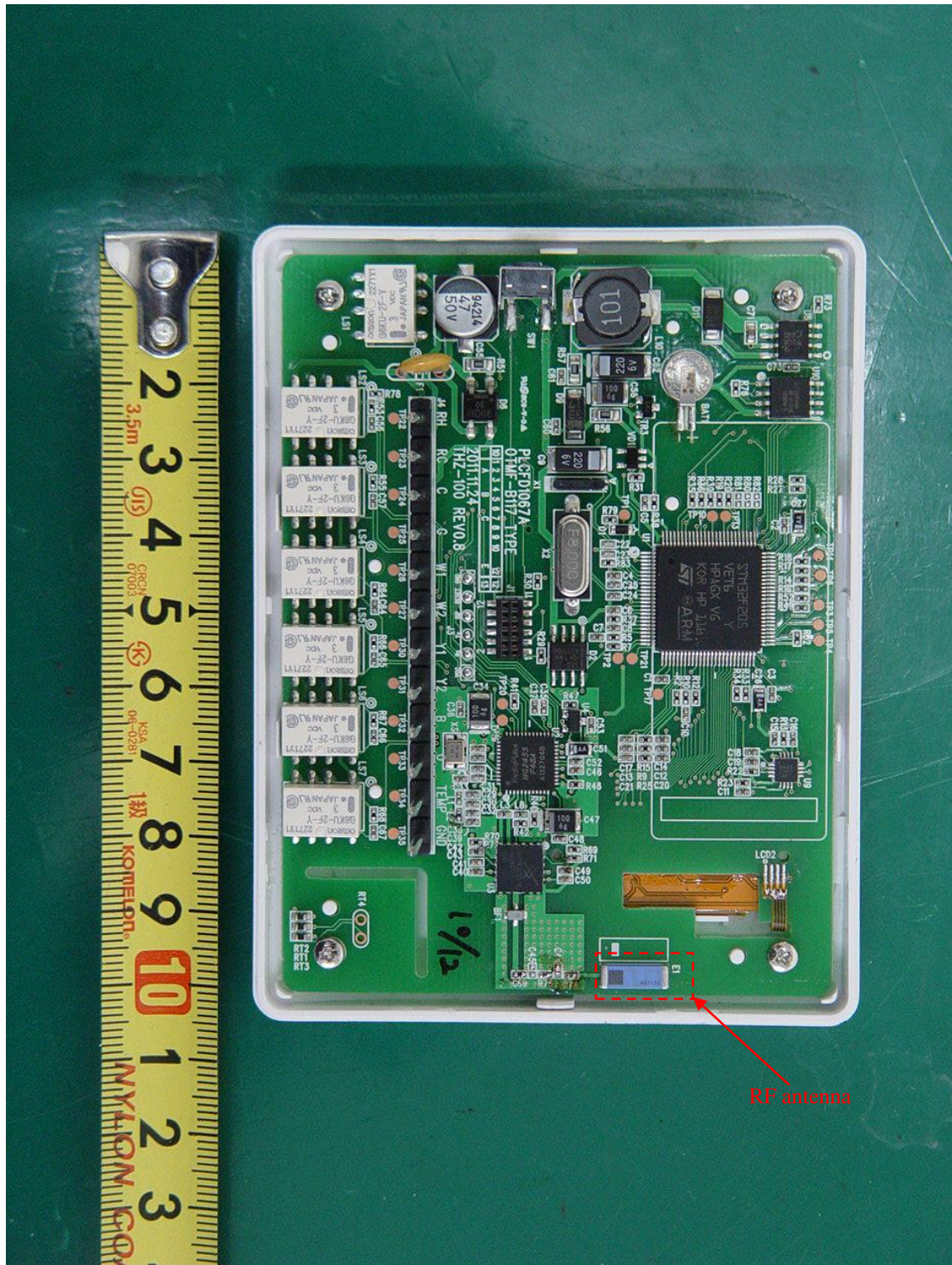
< Inside & main board rear >
