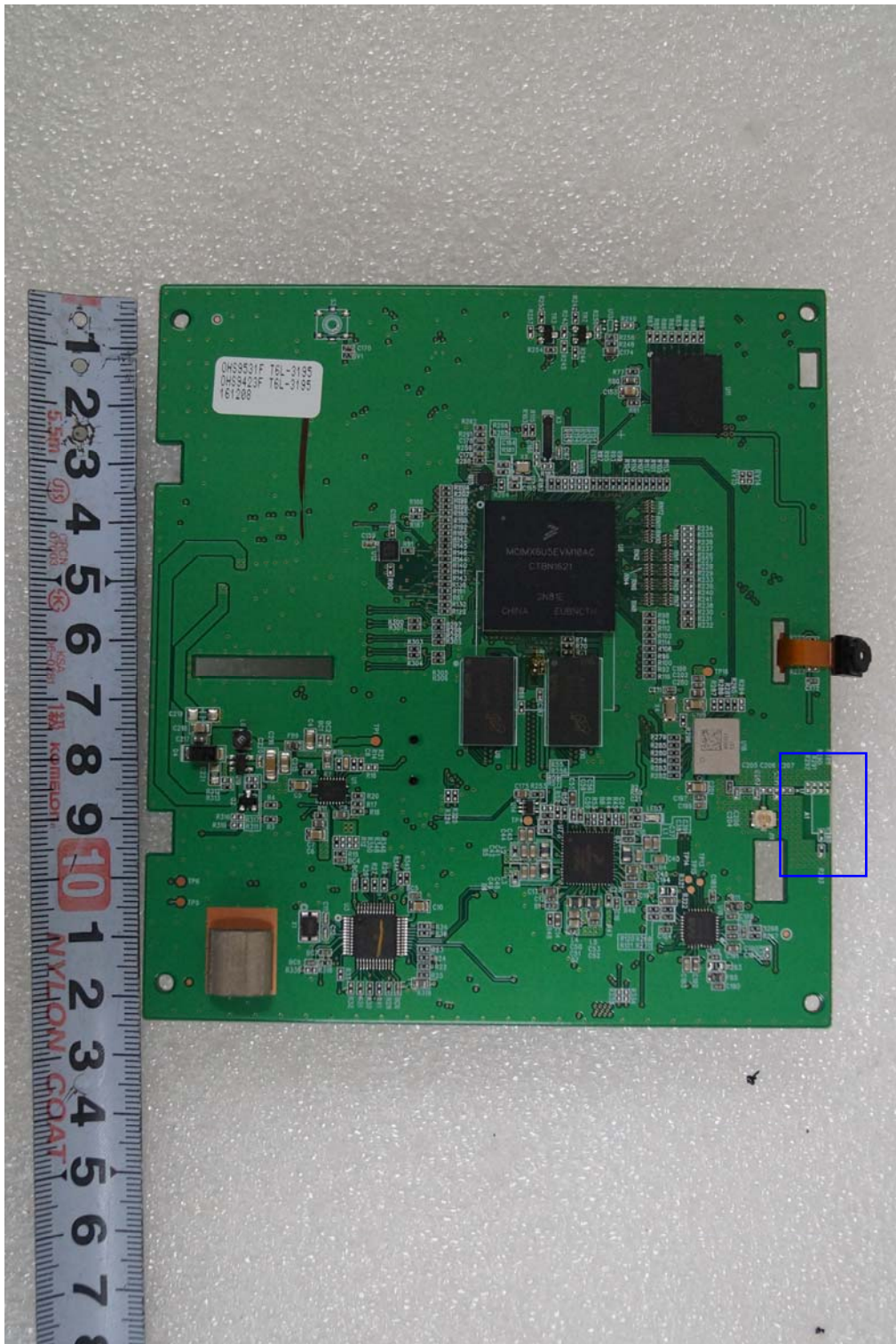
< Original Antenna : Removed Part of Ant impedance matching >
