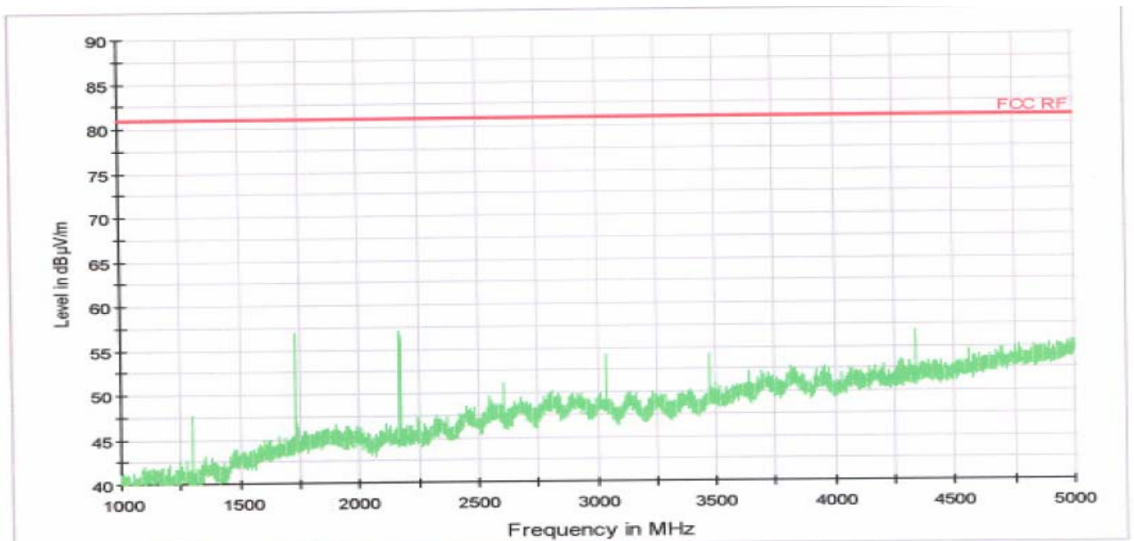
< Fig 5. Radiated Emission result (1000MHz ~ 5000MHz)>
