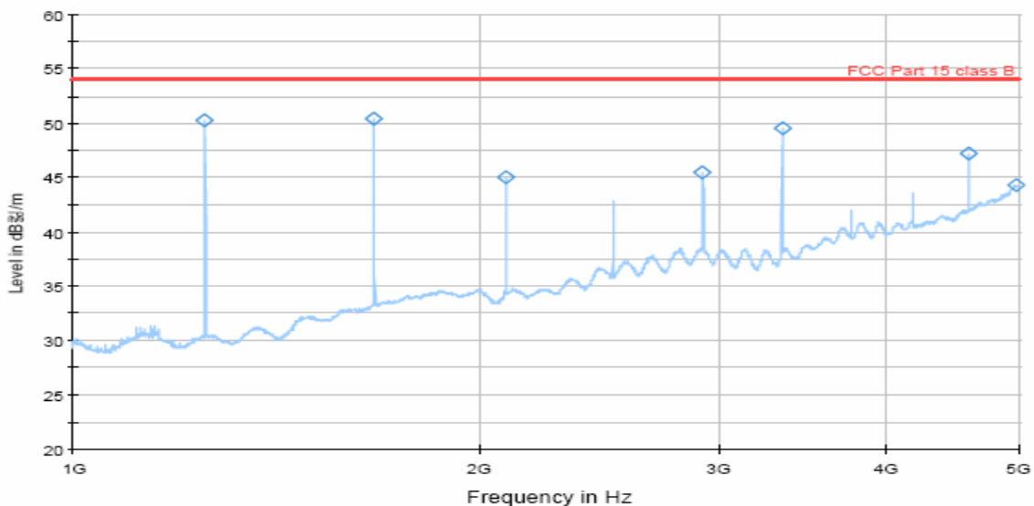
< Fig 5. Radiated Emission result (1000MHz ~ 5000MHz)>
