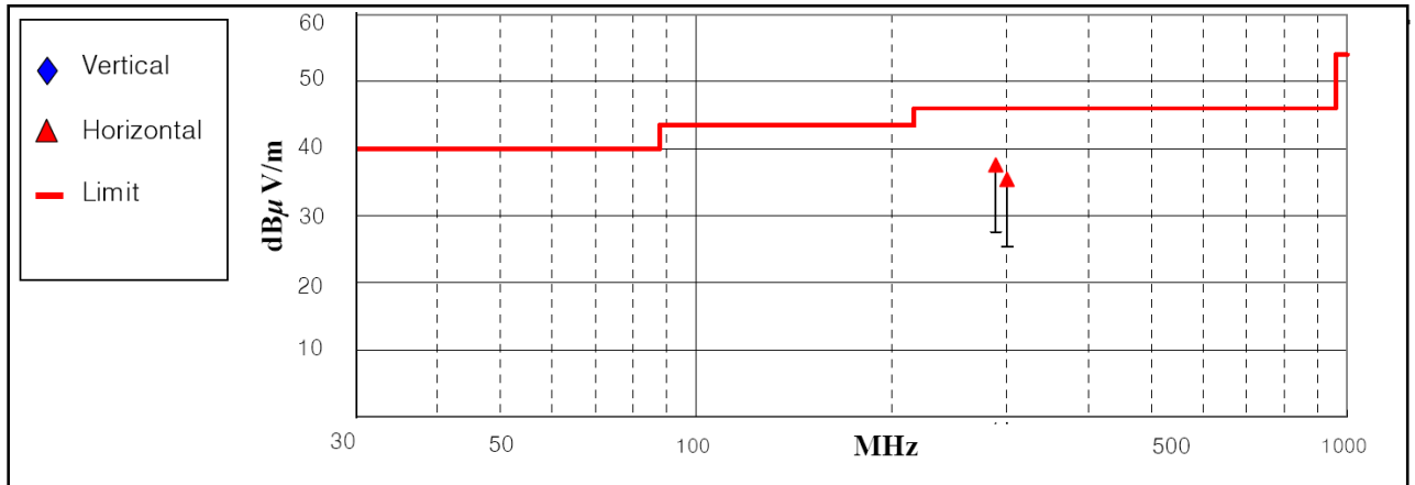
< Fig 6. Radiated emission result (30 MHz ~ 1 000 MHz) >
