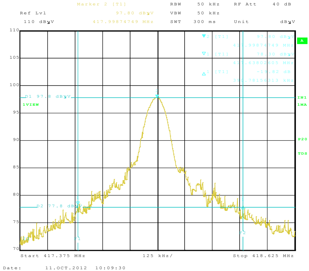
< Fig 9. Occupied bandwidth >
