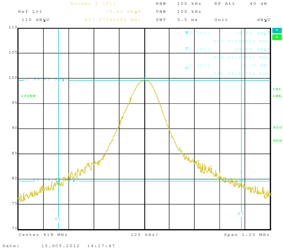
< Fig 9. Occupied bandwidth >
