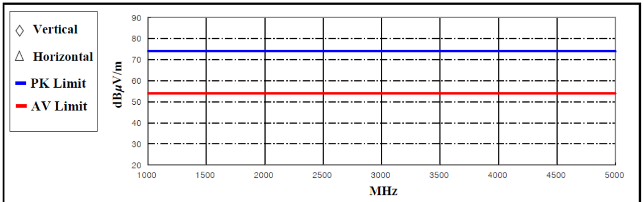
< Fig 8. Radiated emission result (1 GHz ~ 5 GHz) >
