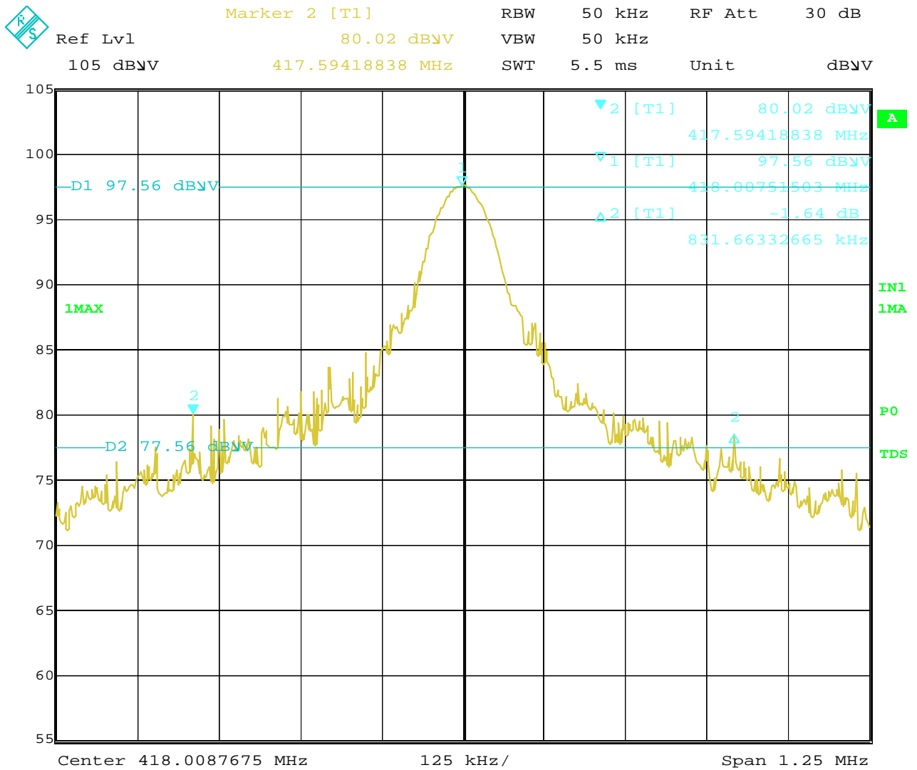
< Fig 7. Occupied bandwidth >
