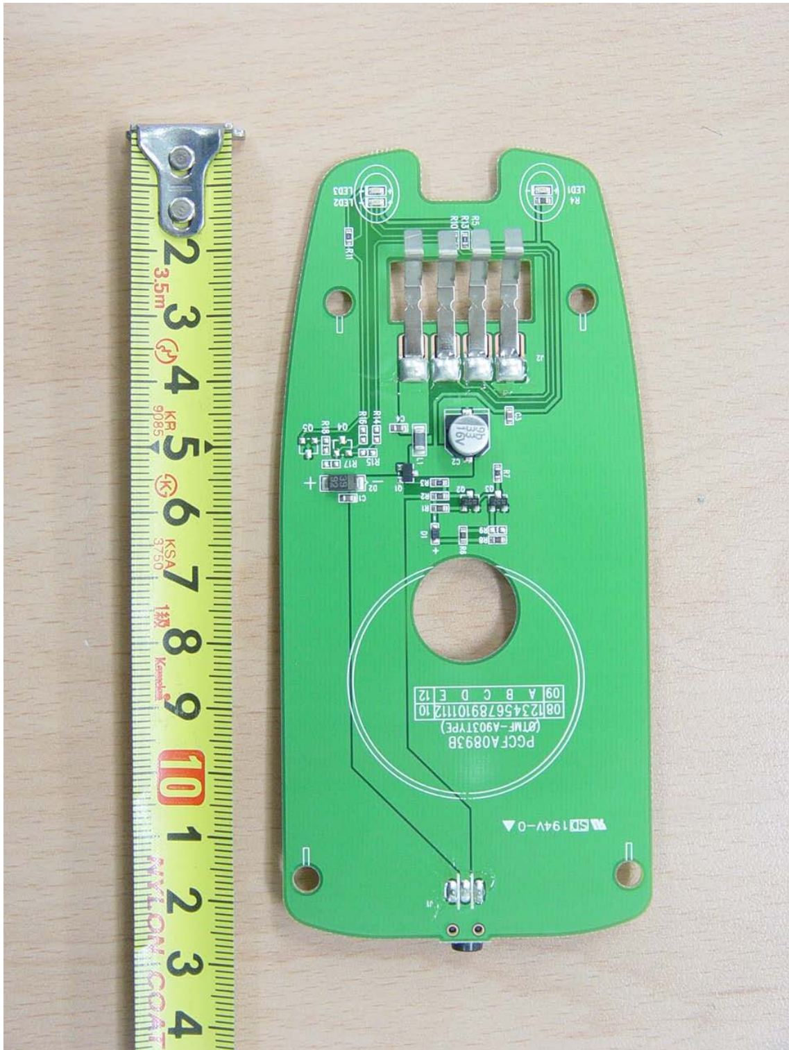
<Charging cradle>
