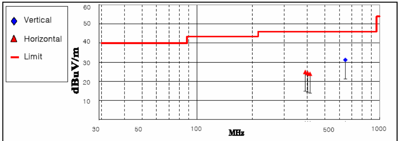
< Fig 5. Radiated emission result (30MHz ~ 1000MHz)_IR mode >
