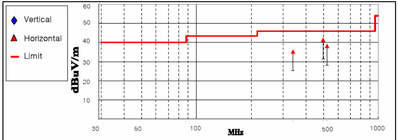
< Fig 3. Radiated emission result (30MHz ~ 1000MHz)_RF mode >
