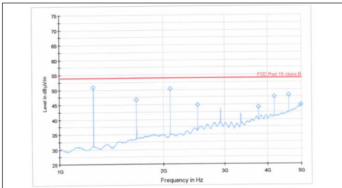
< Fig 4. Radiated Emission result (1000MHz ~ 5000MHz)_RF mode>
