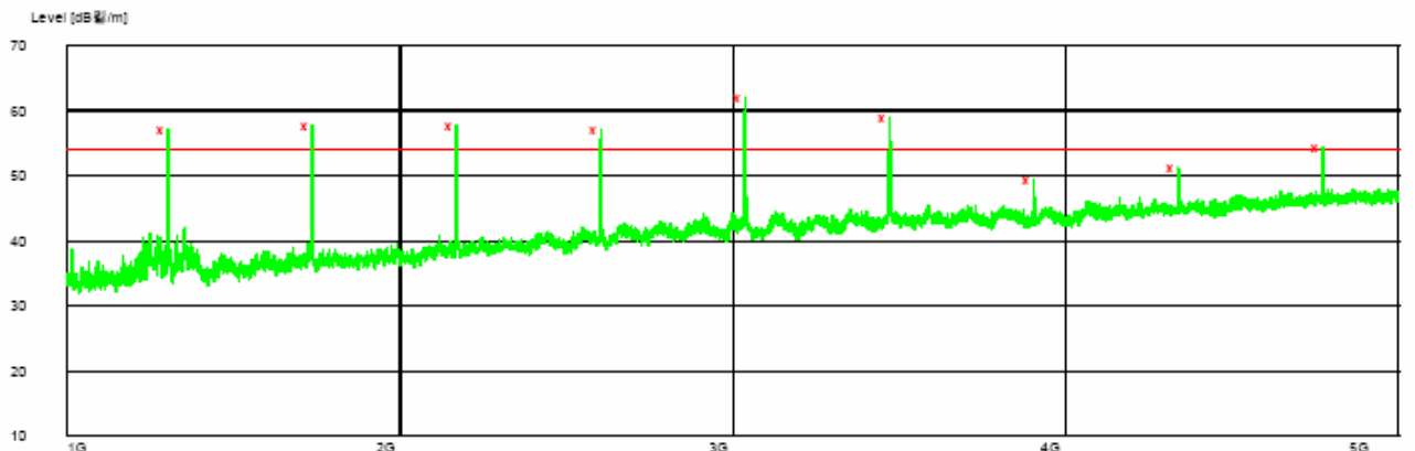
< Fig 5. Radiated Emission result (1000MHz ~ 5000MHz) >
