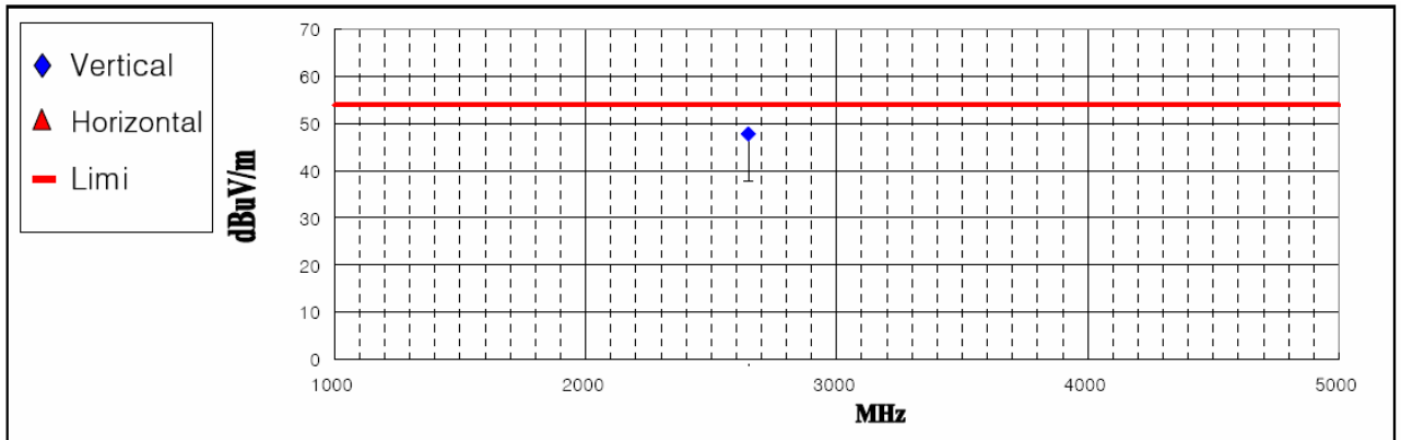
< Fig 6. Radiated Emission result (1000MHz ~ 5000MHz)>
