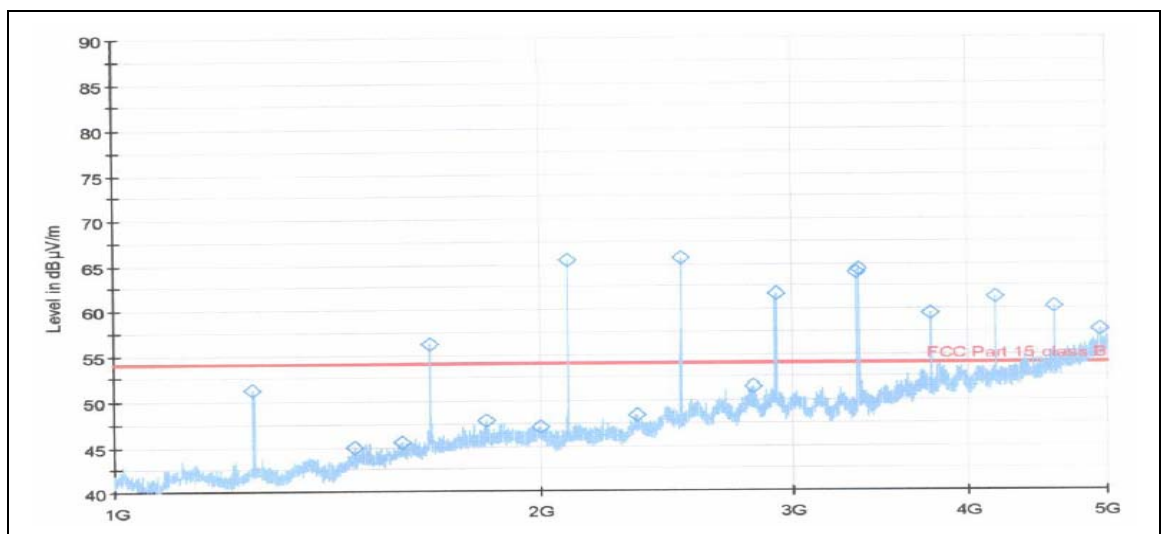
< Fig 5. Radiated Emission result (1000MHz ~ 5000MHz)>
