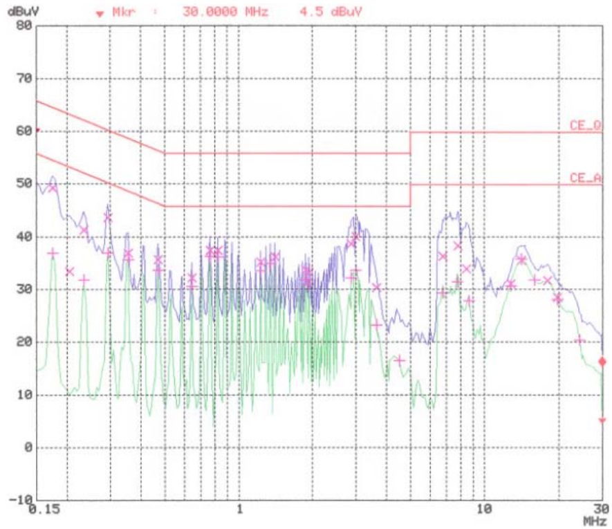
< Hot line >
