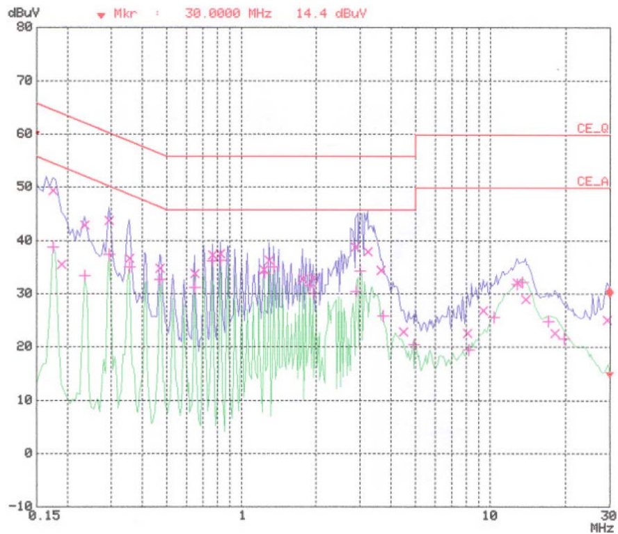
< Neutral line >
