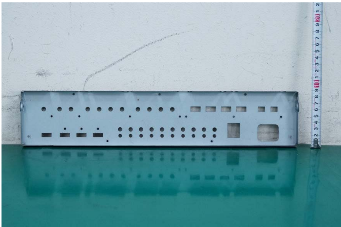
<Rear Frame 2>
