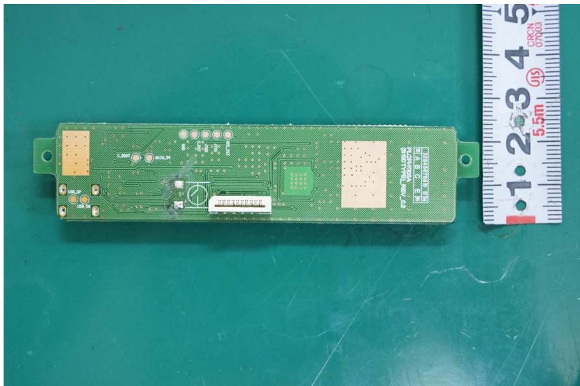
<RF Board Rear>
