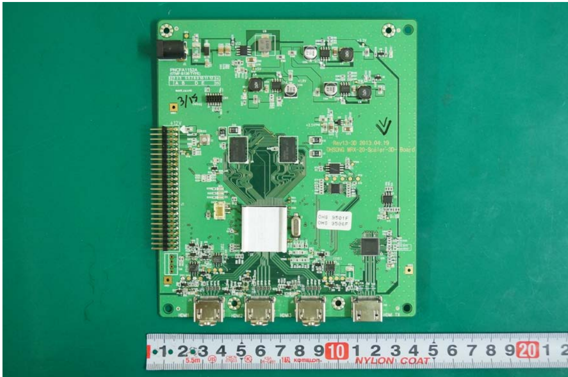
<Network board Front>
