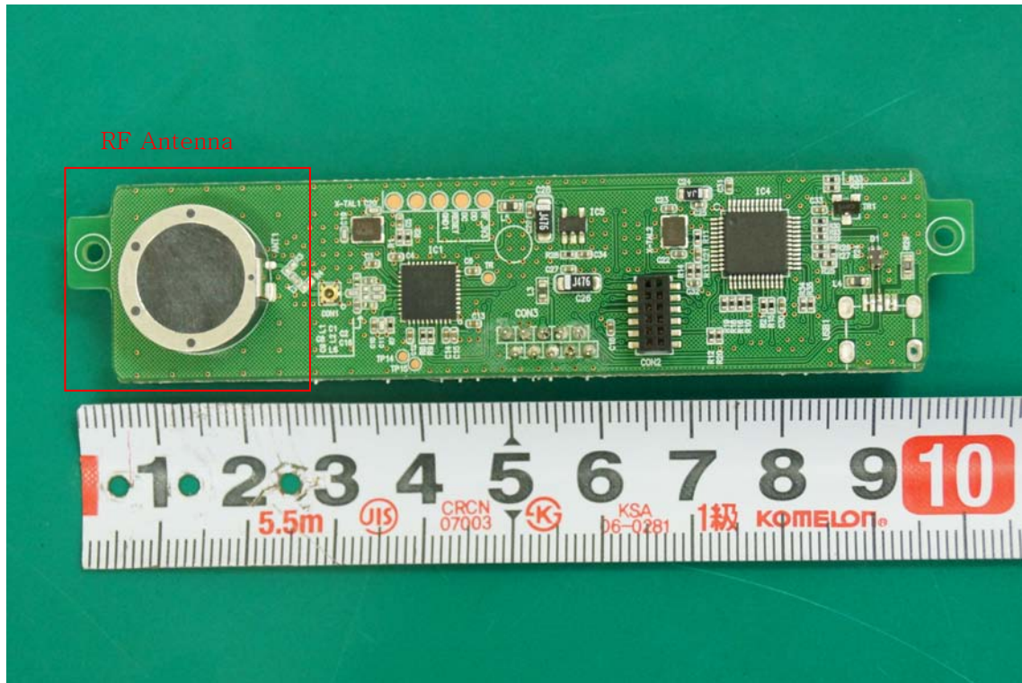
<RF Board Front>
