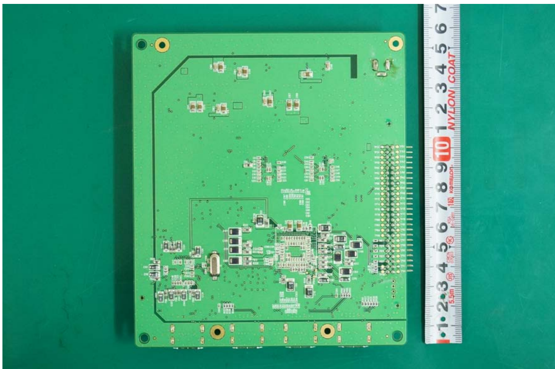
< Network board Rear>
