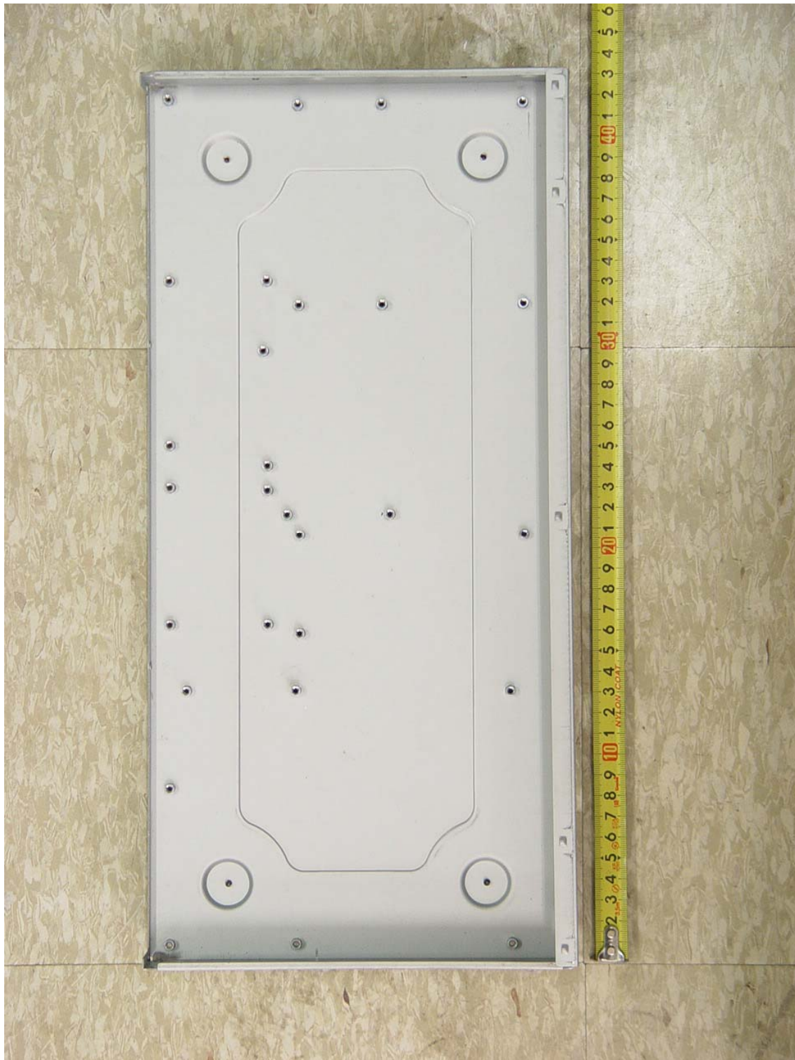
< Shield #2 Rear >
