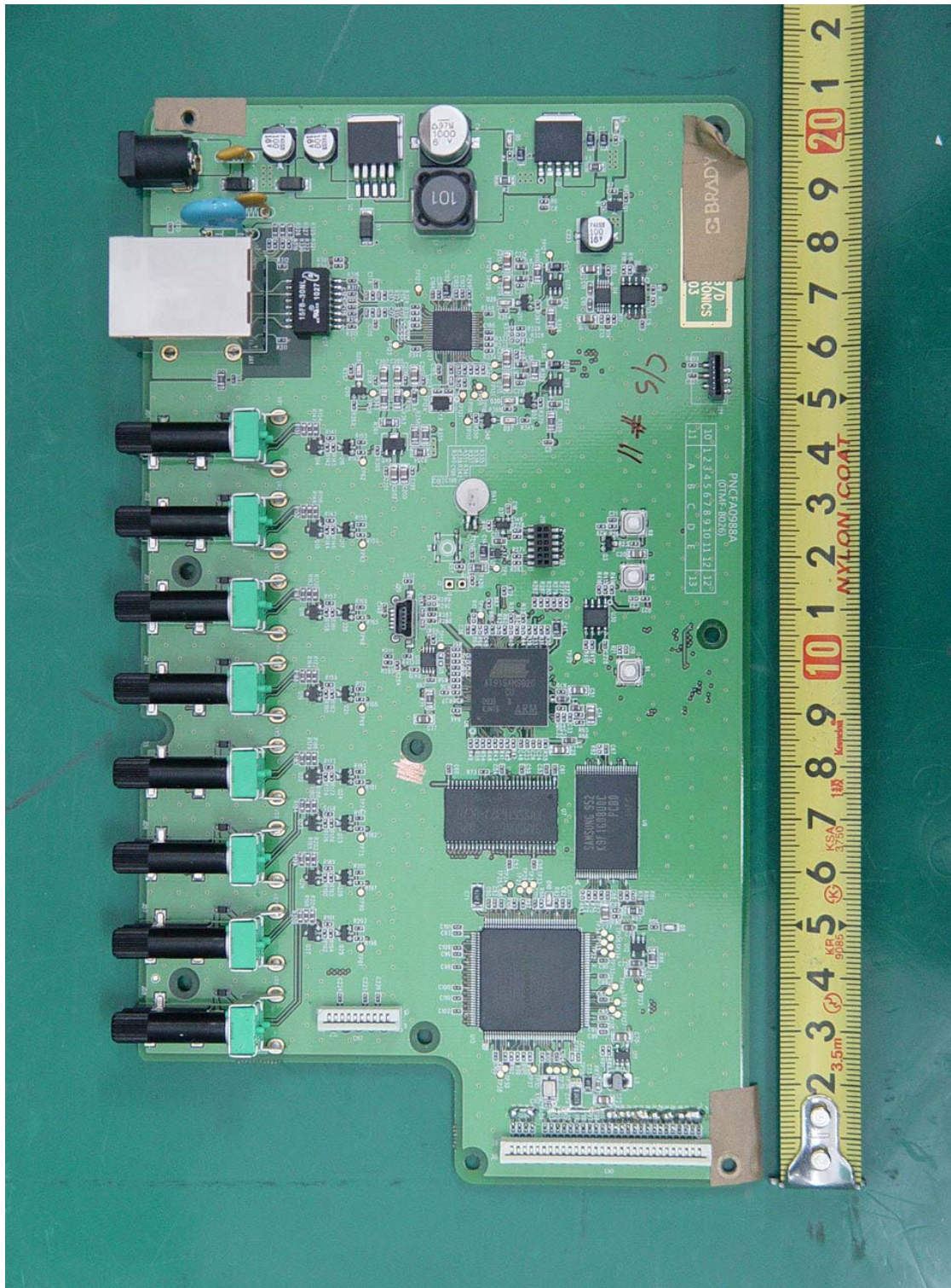
< Board #1 Front >
