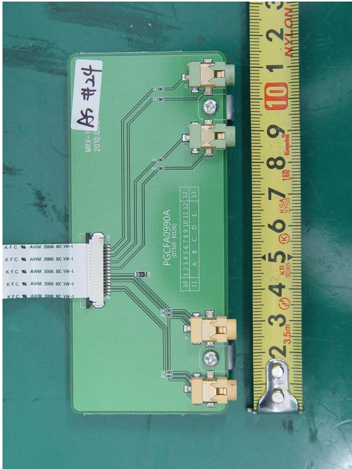
< Board #3 Front >
