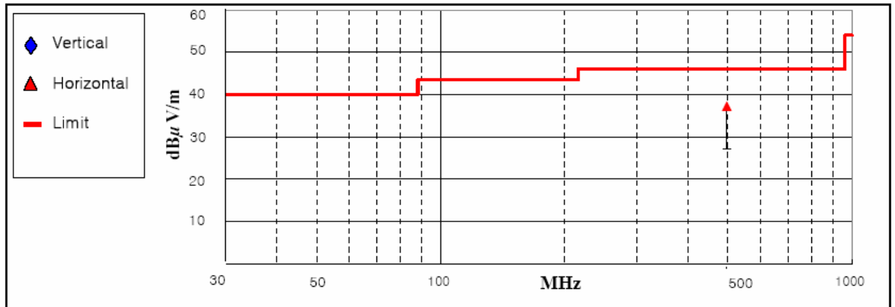
< Fig 4. Radiated emission result >
