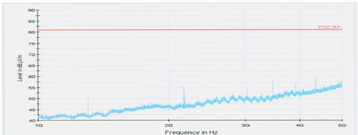
< Fig 5. Radiated Emission result (1000MHz ~ 5000MHz)>
