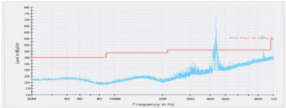
< Fig 4. Radiated emission result (30MHz ~ 1000MHz) >
