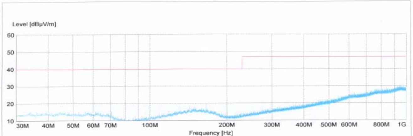
< Fig 4. Radiated emission result (30MHz ~ 1000MHz) >
