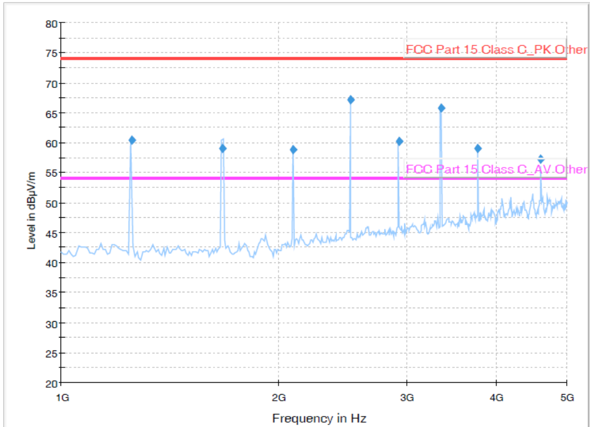
Radiated Emission_above 1 GHz
