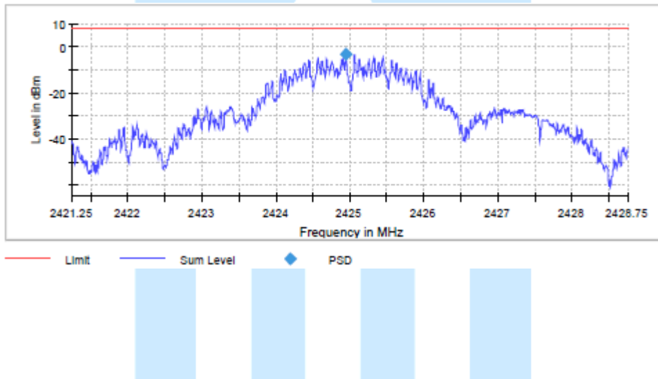
Power Density Plot on configuration : Lowest channel (2 425 MHz)
