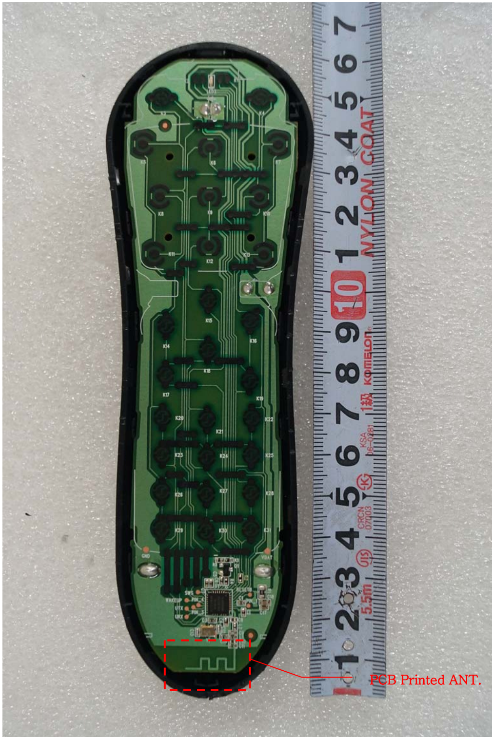
< Location of Antenna >
