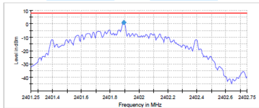
Power Density Plot on configuration : Lowest channel (2 402 MHz)
