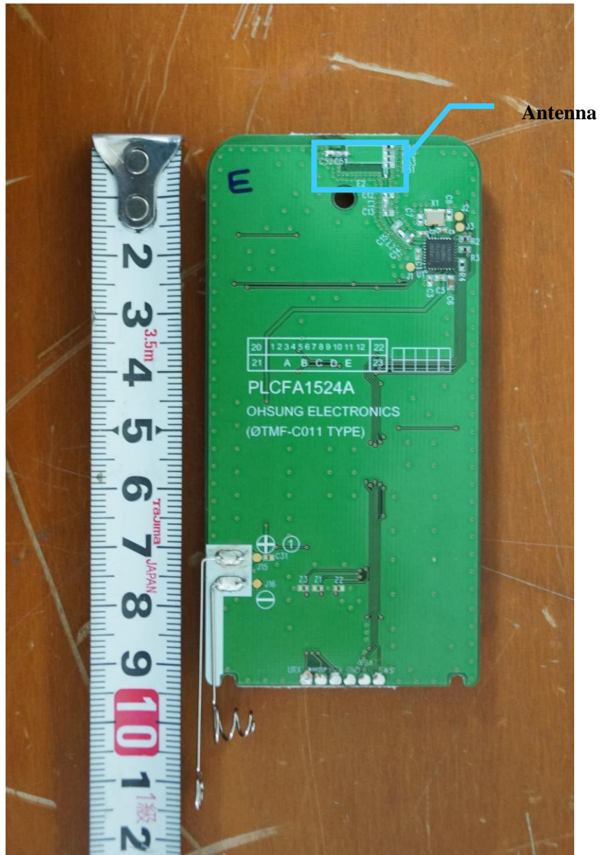
< Main board bottom view >
