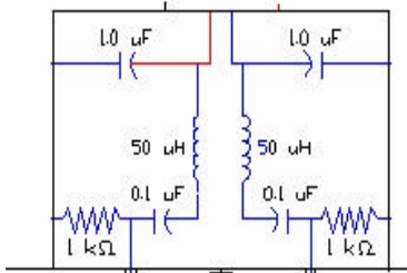
Figure 5. LISN Schematic Diagram
