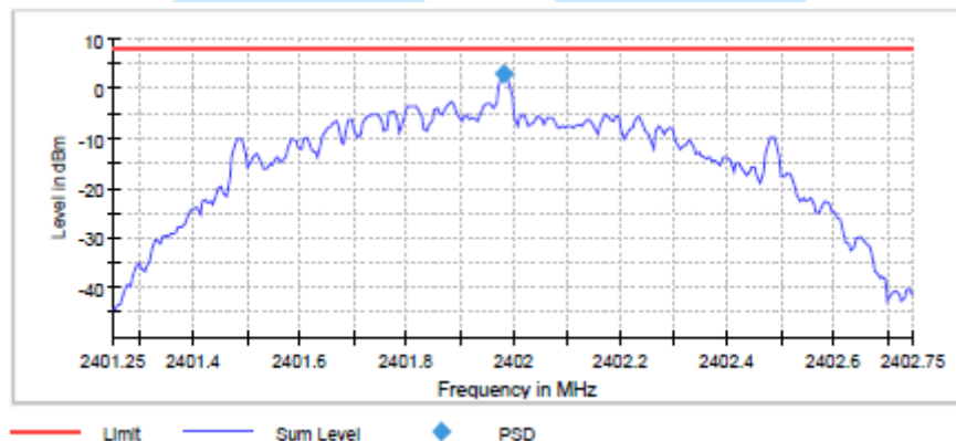
Power Density Plot on configuration : Lowest channel (2 402 MHz)
