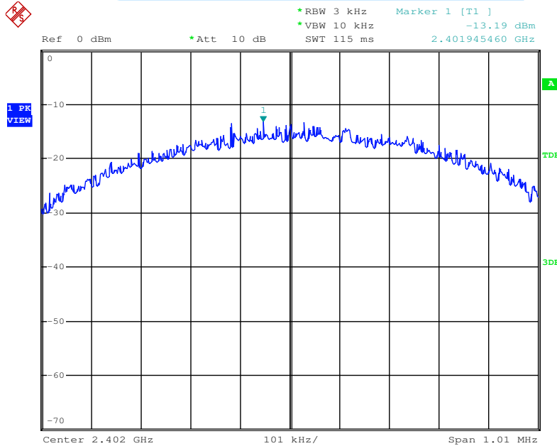
Power Density Plot on configuration : 0ch
