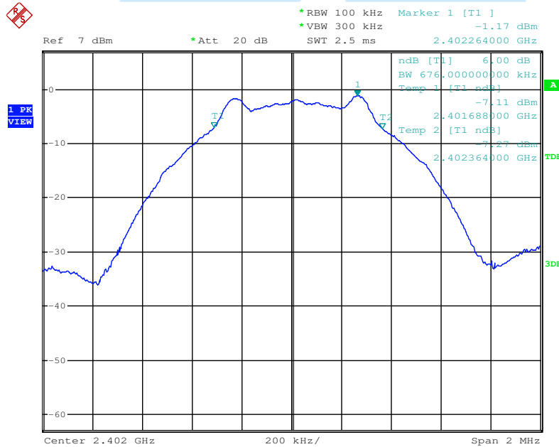
6 dB Bandwidth Plot on Configuration : 0ch
