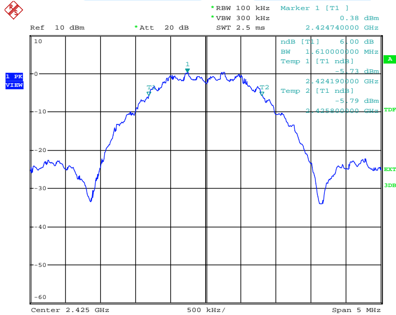
6 dB Bandwidth Plot on Configuration : IEEE 802.15.4 15ch
