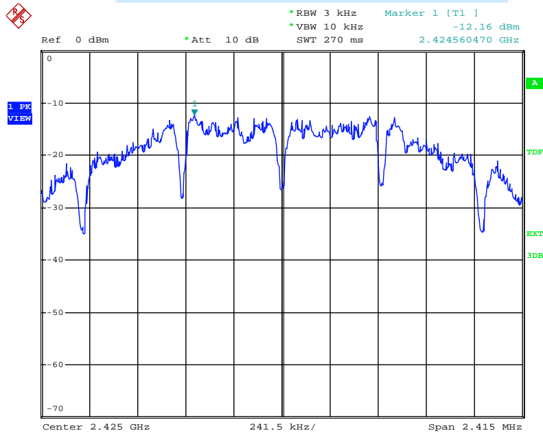
Power Density Plot on configuration : IEEE 802.15.4 15ch
