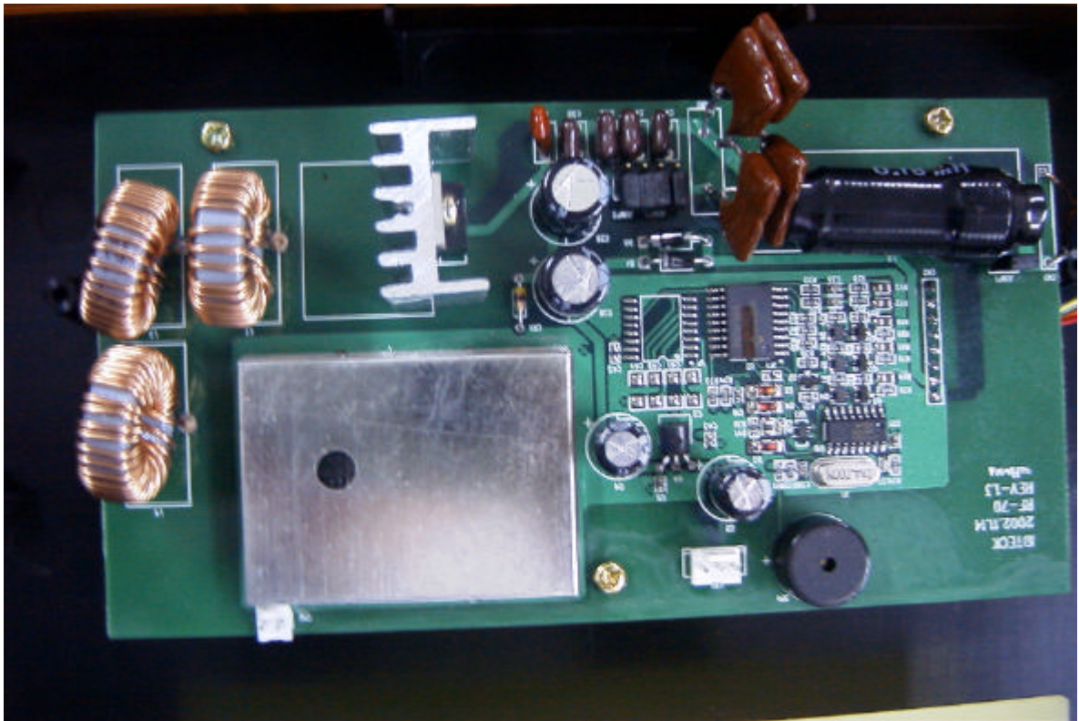
[ Main PCB Top View ]
