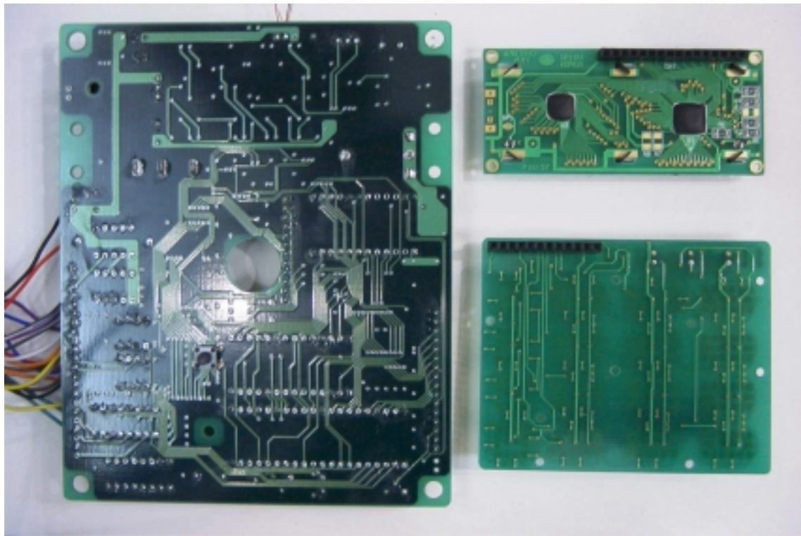
<Bottom View>
