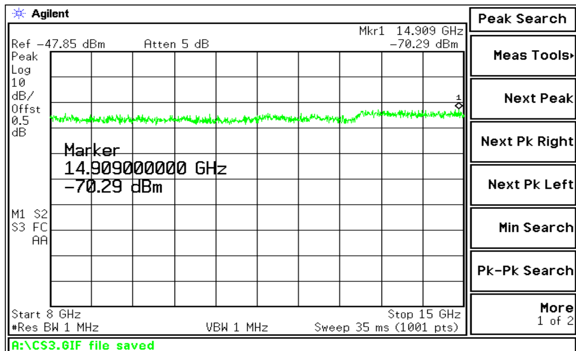
(Out of band Conducted Emissions, 8 GHz ~ 15 GHz)
