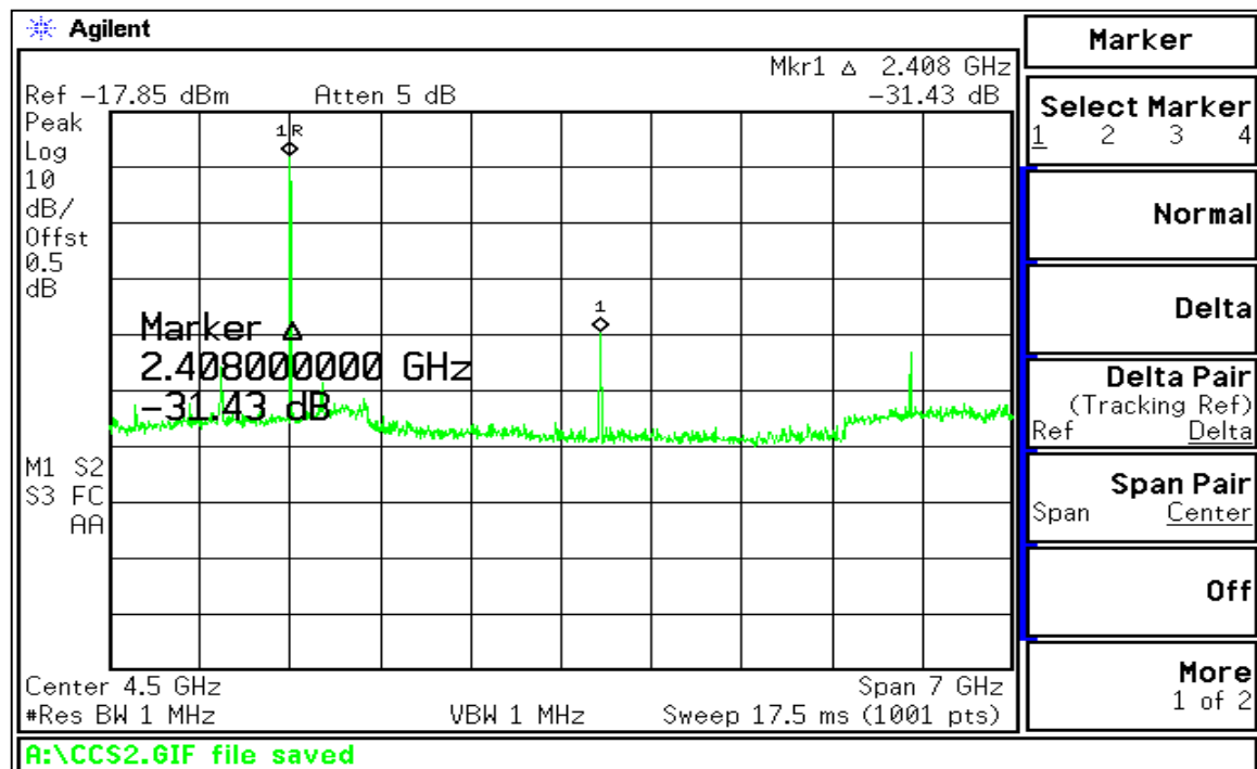
(Out of band Conducted Emissions, 1 GHz ~ 8 GHz)
