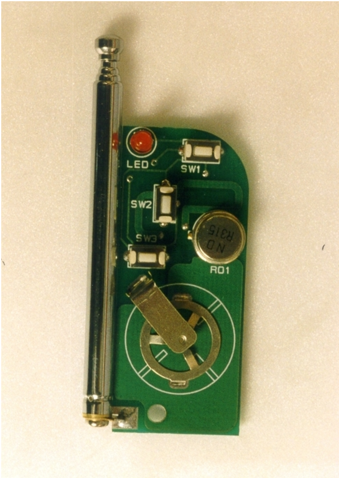
<Front Side of PCB>
