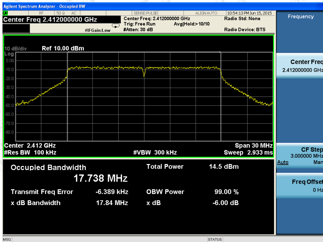
802.11n HT20 channel, 6dB bandwidth / ANT_2
