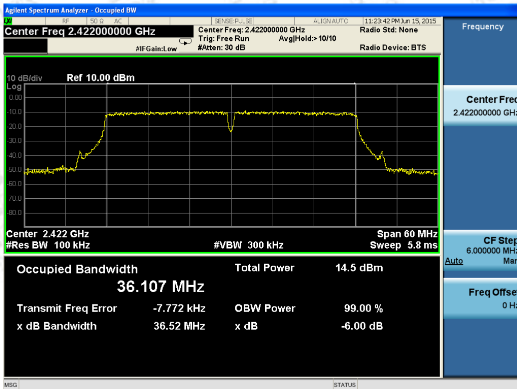
802.11n HT40 channel, 6dB bandwidth / ANT_2
