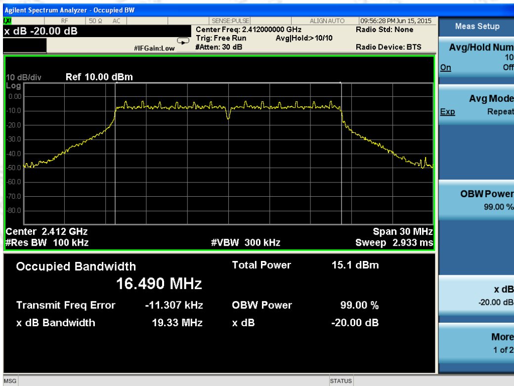
802.11g channel, 20dB bandwidth / ANT_2
