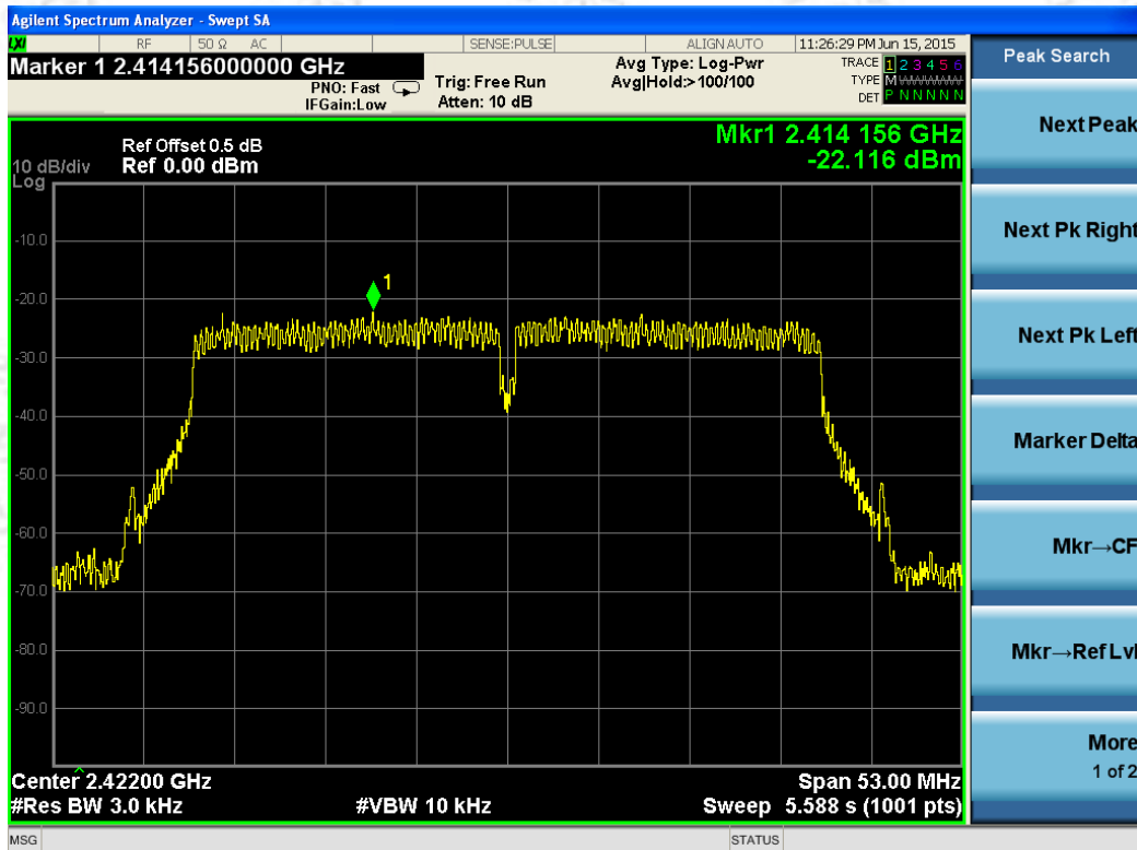
802.11n HT40 power density / ANT_2
