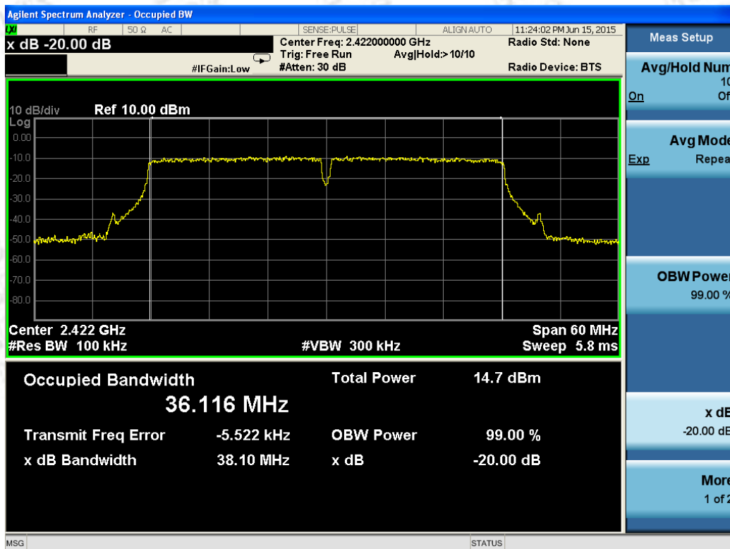
802.11n HT40 channel, 20dB bandwidth / ANT_2
