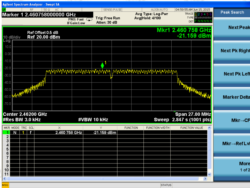
802.11n HT20 power density / ANT_2
