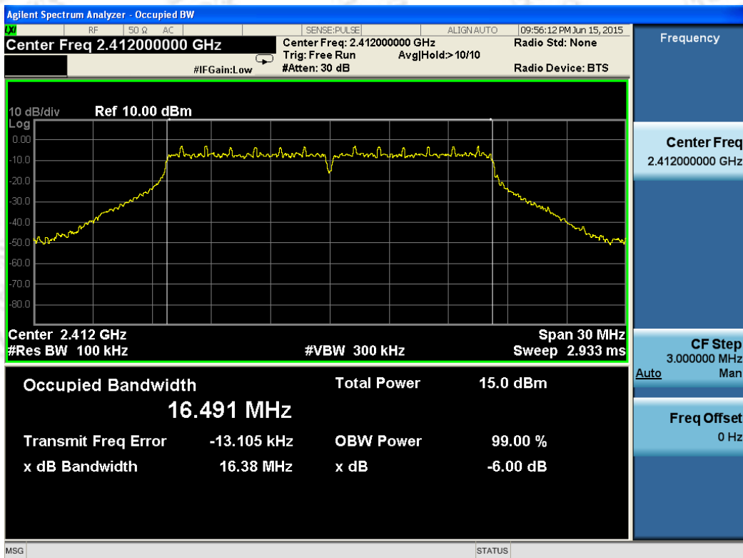
802.11g channel, 6dB bandwidth / ANT_2
