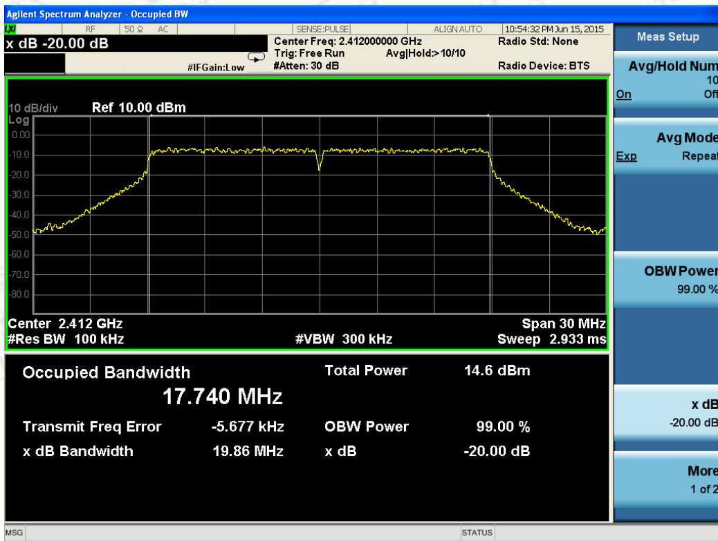
802.11n HT20 channel, 20dB bandwidth / ANT_2
