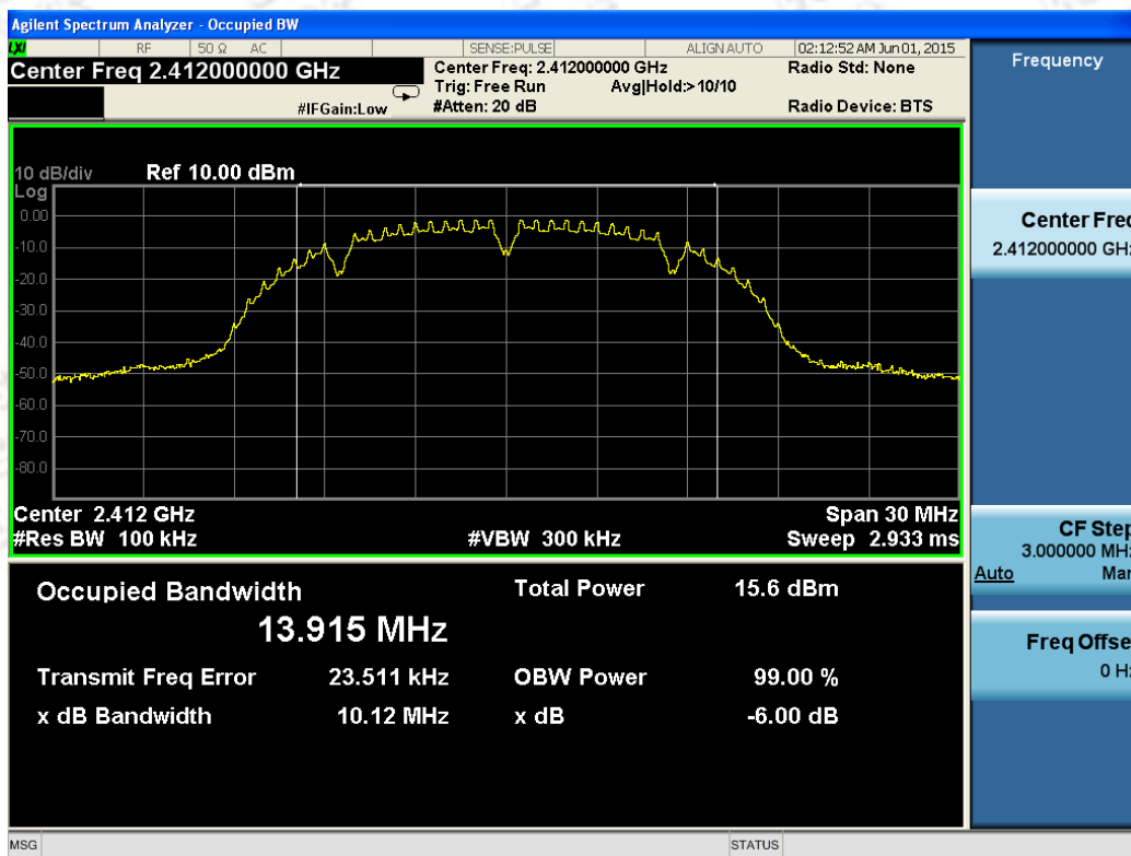
802.11b channel, 6dB bandwidth / ANT_2
