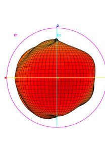
Total_3D_E1_2.45GHz
