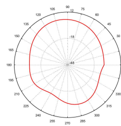
Total_Polar_E2_2.45GHz
