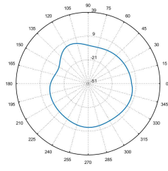
Total_Polar_E1_5.55GHz
