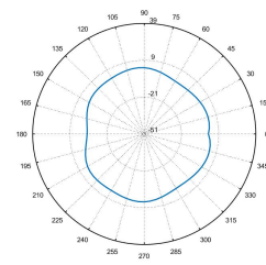
Total_Polar_E2_5.55GHz
