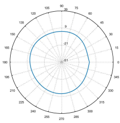
Total_Polar_H_5.55GHz
