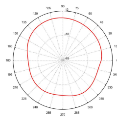
Total_Polar_H_2.5GHz
