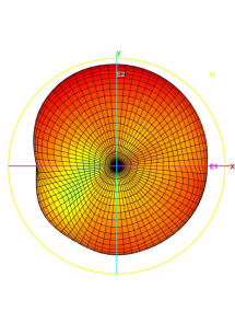
Total_3D_H_2.45GHz
