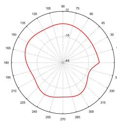
Total_Polar_E1_2.45GHz
