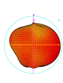
Total_3D_E2_2.45GHz
