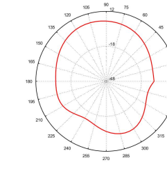
Total_Polar_E2_2.5GHz
