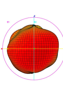
Total_3D_E1_2.5GHz
