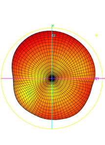
Total_3D_H_2.5GHz
