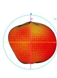
Total_3D_E2_2.5GHz
