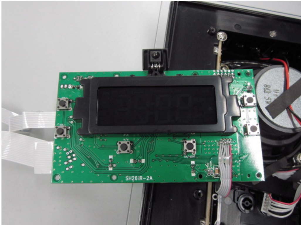
1.1.19 Rear view
