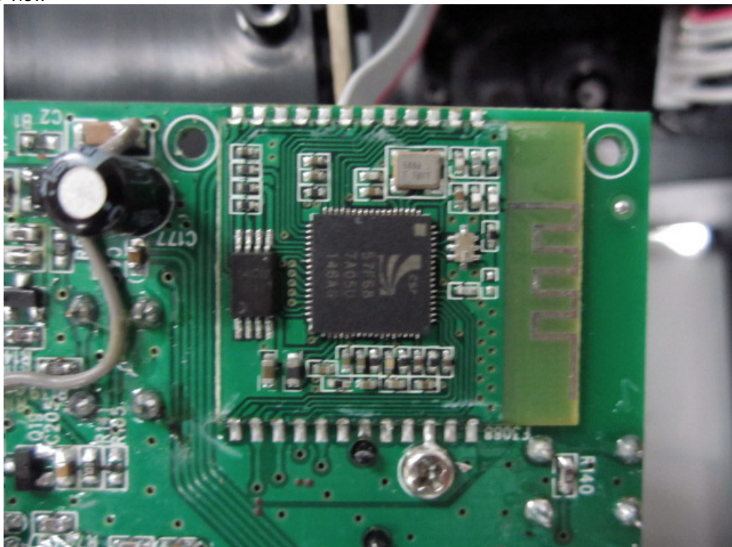
1.1.18 Rear view
