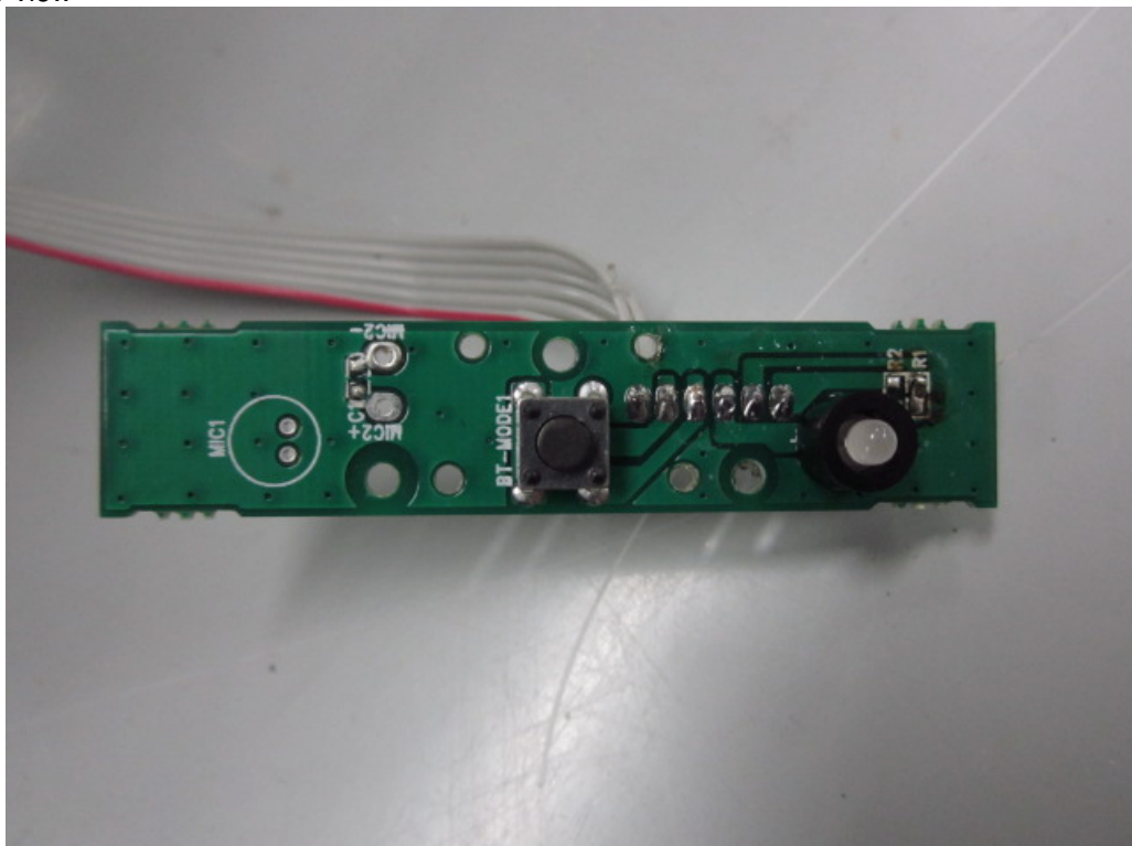
1.1.26 Rear view
