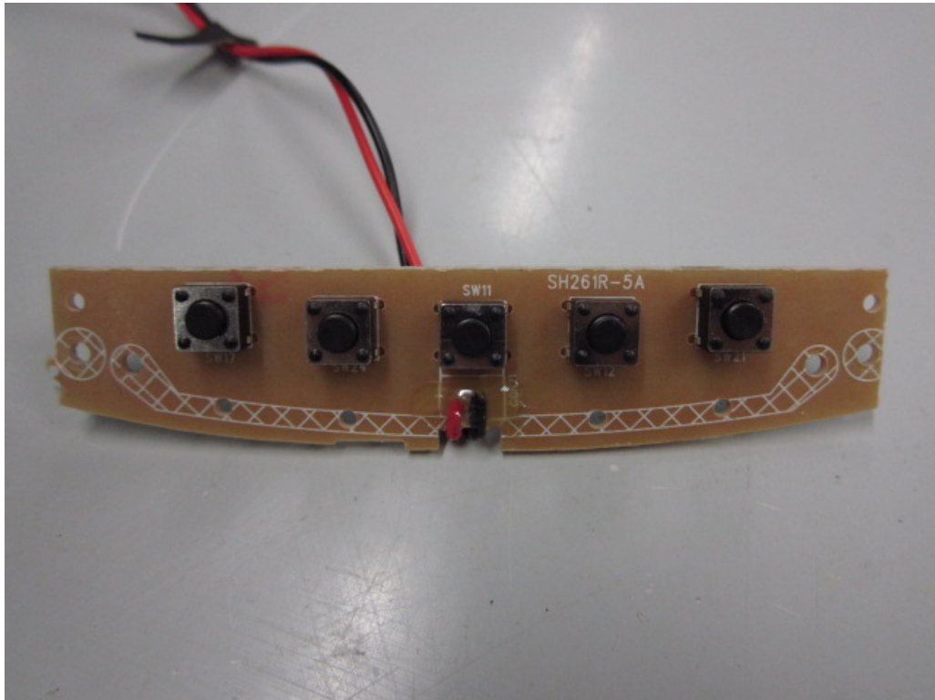
1.1.29 Rear view
