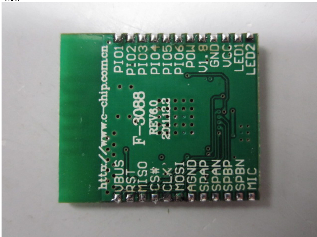
1.1.32 Rear view
