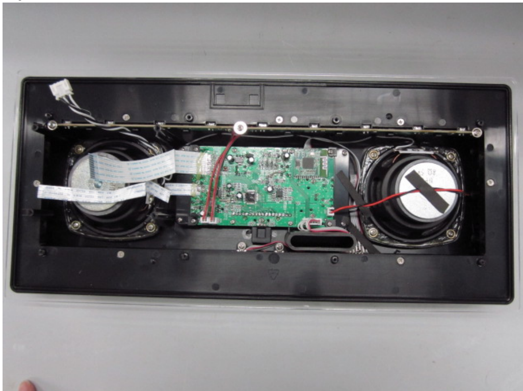
1.1.16 Rear view
