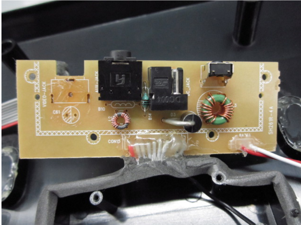
1.1.15 Rear view
