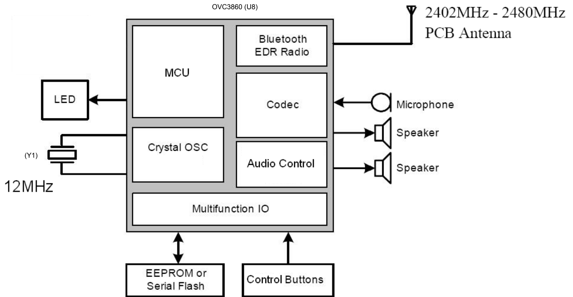
F-3089 Block Diagram
