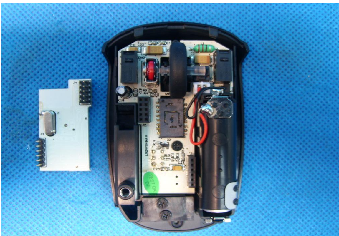
Fig.6 Remove top PCB(L0247075V:C)
